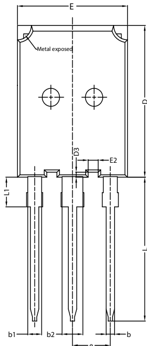
TOP VIEW
