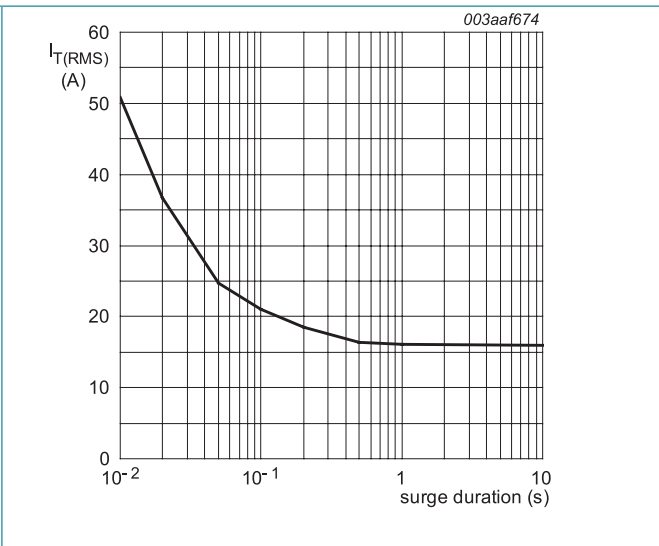
f = 50 \text{ Hz}; T_{mb} = 126 \text{ }^\circ\text{C} Fig. 3. RMS on-state current as a function of surge duration; maximum values
