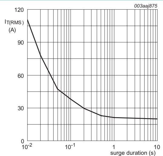
Fig. 2. RMS on-state current as a function of surge duration; maximum values f = 50\text{ Hz} ; T_h = 75\text{ °C}
