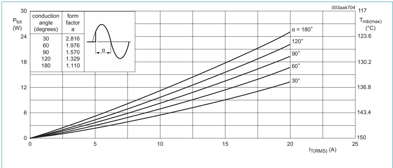
\alpha = conduction angle Fig. 3. Total power dissipation as a function of RMS on-state current; maximum values
