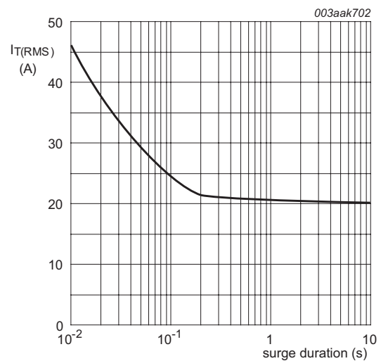
f = 50\text{ Hz} ; T_{mb} = 122\text{ °C} Fig. 2. RMS on-state current as a function of surge duration; maximum values
