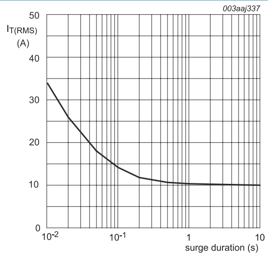
f = 50\text{ Hz} ; T_{mb} = 131\text{ °C} Fig. 2. RMS on-state current as a function of surge duration; maximum values
