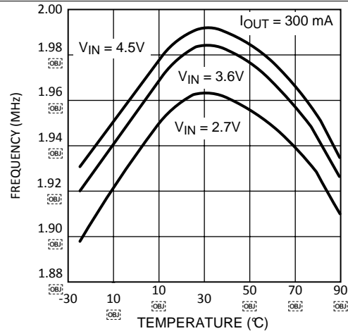
Figure 8. Switching Frequency vs Temperature
