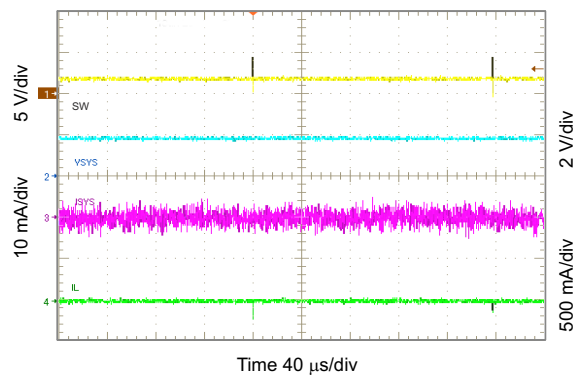
Figure 10-24. 3.3 V sys Line Regulation
