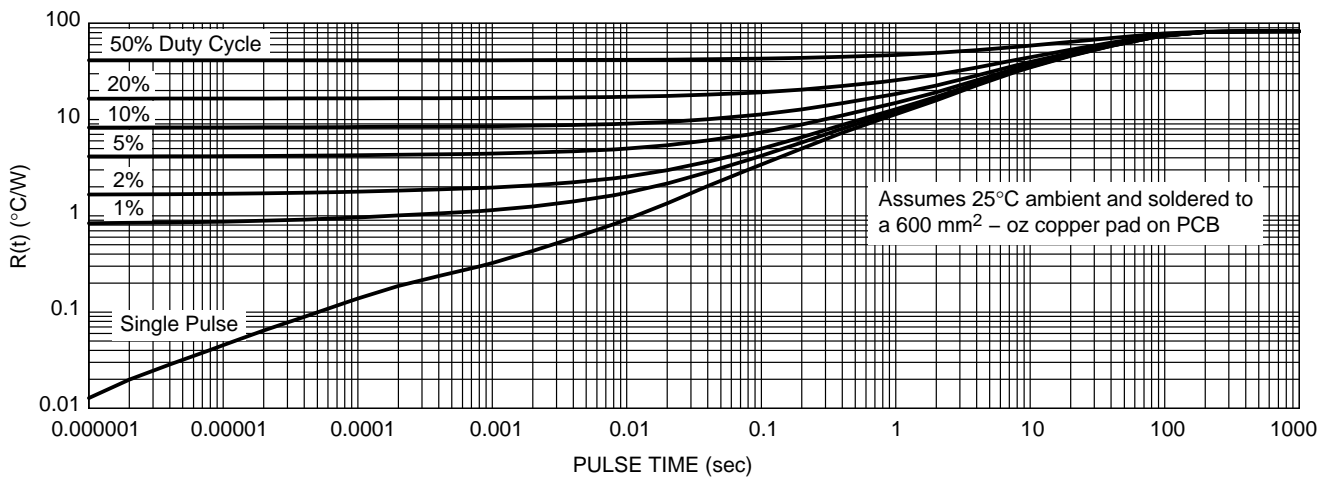
Figure 8. Thermal Characteristics
