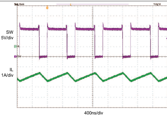
Figure 44. PWM Switching Waveform
