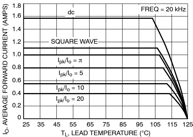
Figure 5. Current Derating
