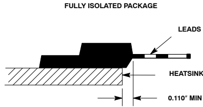
Figure 3. Mounting Position
