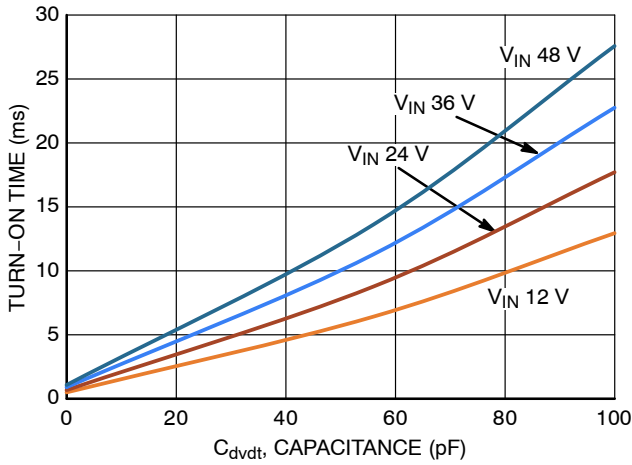
Figure 7. Turn-on Time vs. C_{dvdt} Capacitance at T_J = -40^\circ\text{C}
