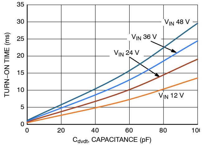
Figure 8. Turn-on Time vs. C_{dvdt} Capacitance at T_J = 25^\circ\text{C}
