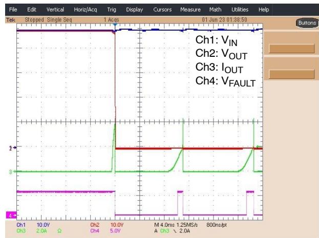
Figure 19. I_{CB} Overcurrent Event on Auto-retry Device
