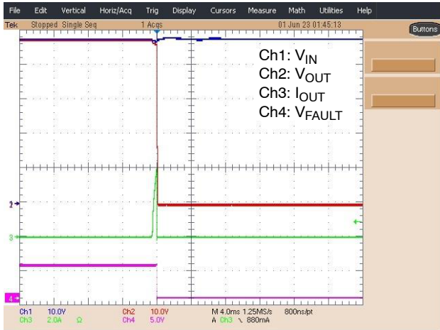
Figure 18. I_{CB} Overcurrent Event on Latching Device
