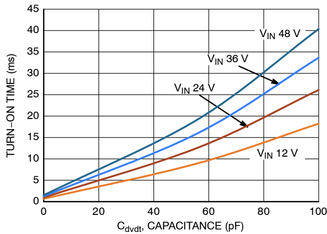
Figure 9. Turn-on Time vs. C_{dvdt} Capacitance at T_J = 125^\circ\text{C}
