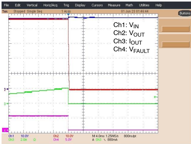
Figure 16. I_{TH} Overcurrent Event on Latching Device
