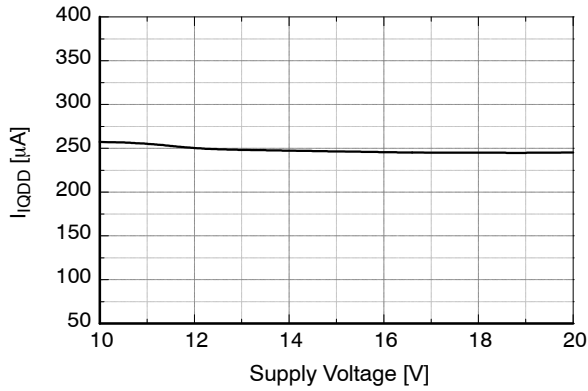
Figure 30. Quiescent V DD Supply Current vs. Supply Voltage
