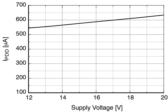
Figure 32. Operating V DD Supply Current vs. Supply Voltage
