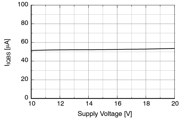
Figure 31. Quiescent V BS Supply Current vs. Supply Voltage
