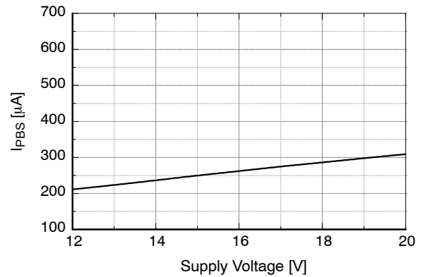
Figure 33. Operating V BS Supply Current vs. Supply Voltage
