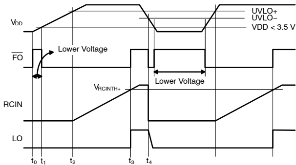
Figure 38. Waveforms for Under-Voltage Lockout
