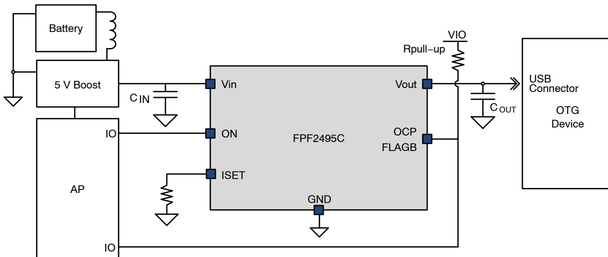
Figure 1. Typical Application
