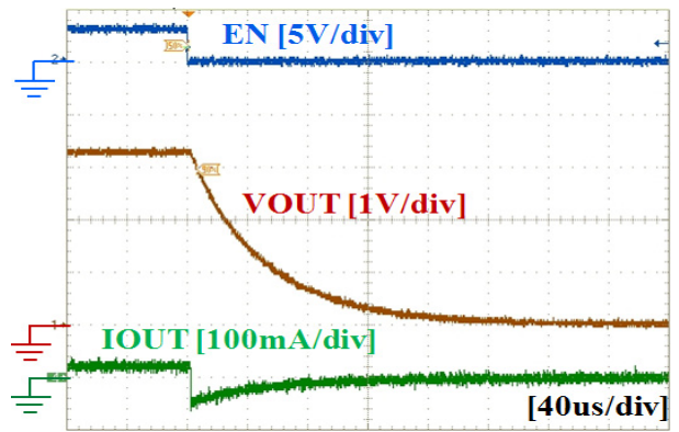
Figure 28. Turn-Off Response with FPF1321 ( V_{IN} = 3.3\text{ V} , C_{IN} = 1\ \mu\text{F} , C_{OUT} = 1\ \mu\text{F} , R_L = 150\ \Omega , SEL = \text{LOW} )
