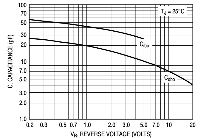
Figure 9. Capacitances
