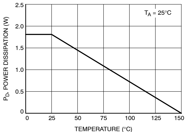
Figure 13. Power Derating
