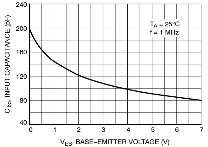
Figure 10. Input Capacitance
