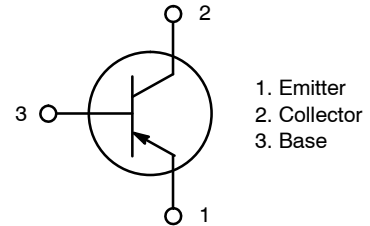
TO-92 3 CASE 135AP
