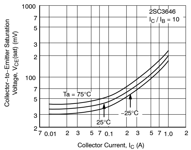
Figure 12. V_{CE(sat)} - I_C
