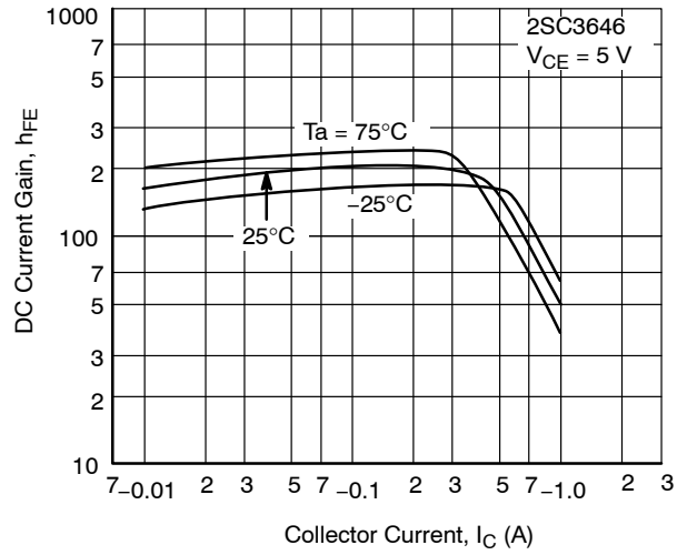
Figure 8. h_{FE} - I_C
