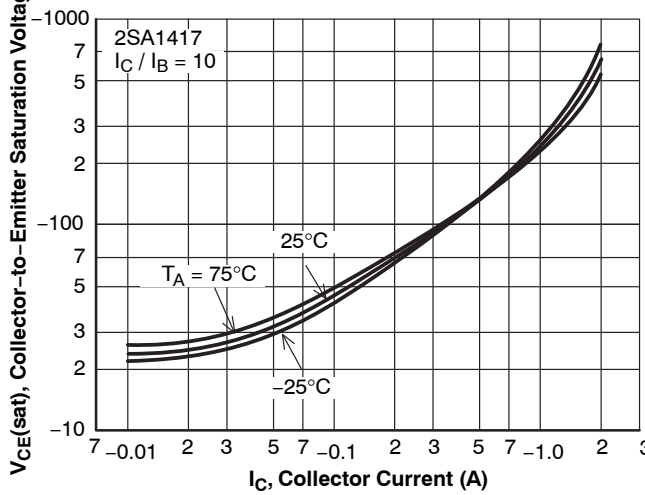
Figure 12. V_{CE(sat)} - I_C
