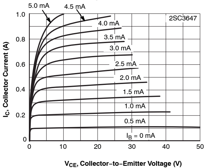
Figure 5. I_C - V_{CE}
