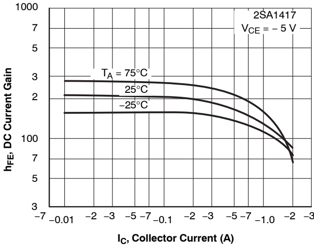
Figure 8. h_{FE} - I_C
