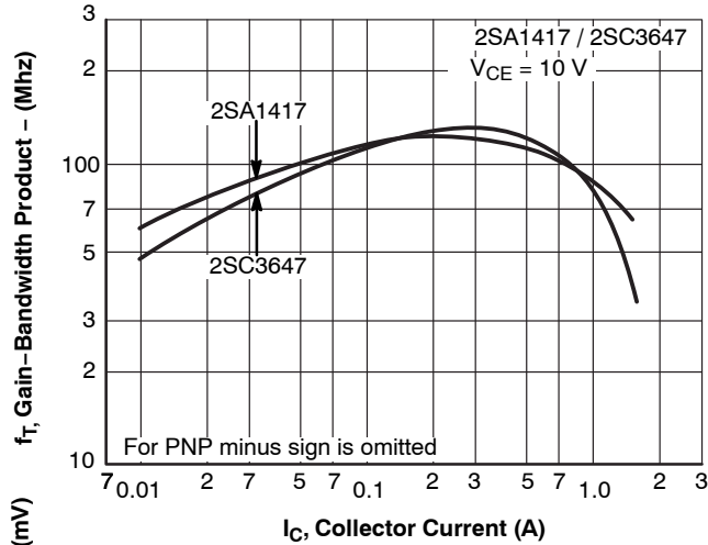
Figure 10. f_T - I_C
