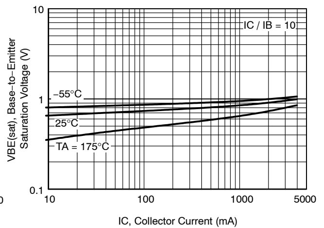
Figure 7. V_{BE(sat)} - I_C
