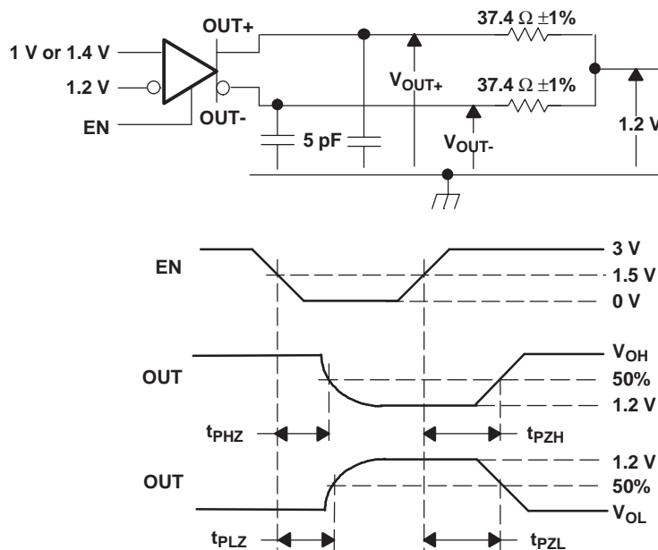
Figure 5. Timing Test Circuit and Waveforms
