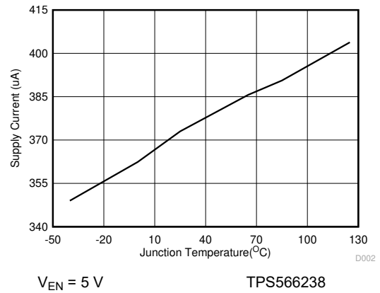
Figure 6-2. Supply Current vs Junction Temperature
