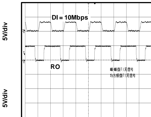
Time (100ns/div)
