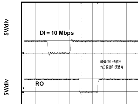
Time (100ns/div)
