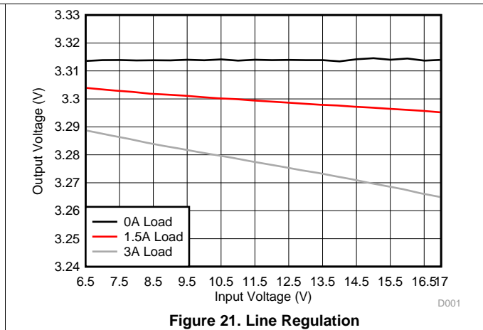
Figure 21. Line Regulation
