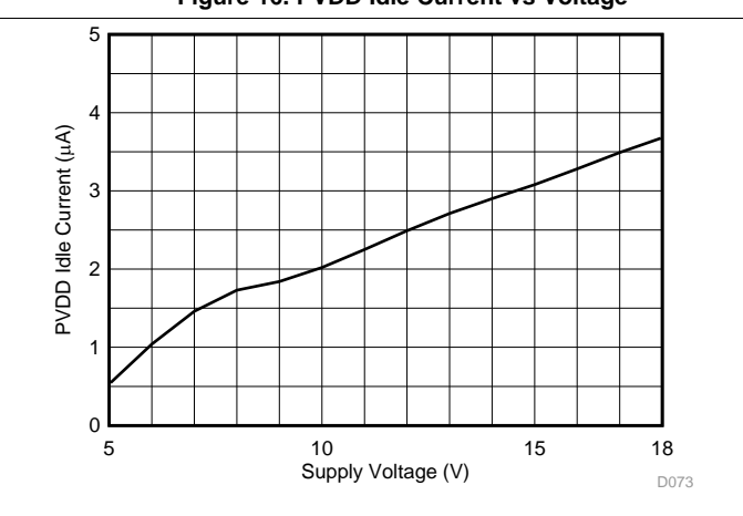
Figure 18. PVDD Standby Current vs Voltage
