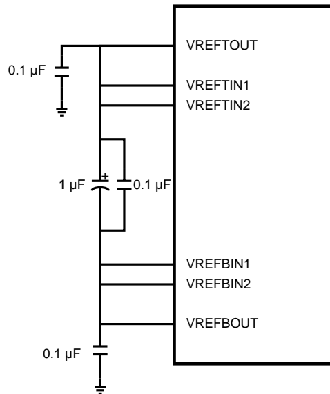
Figure 23. Reference Decoupling Example
