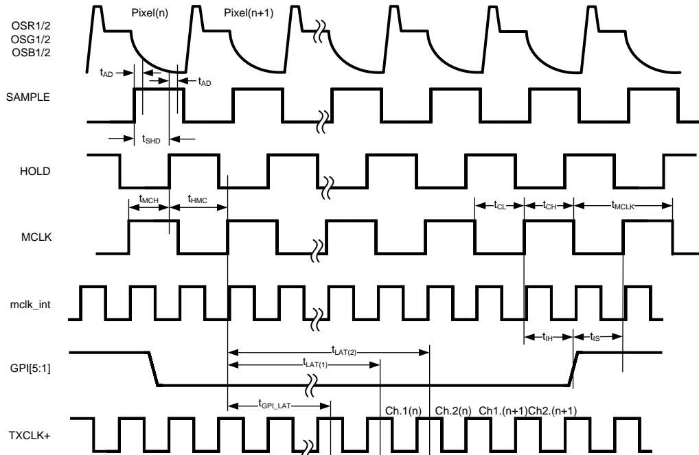
Figure 7. Output Latency and Timing – 6 Channel Mode – Pixel Rate MCLK
