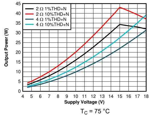
T_C = 75^\circ\text{C} BTL Figure 6-4. Output Power vs Supply Voltage - 2 \Omega 1%, 2 \Omega 10%, 4 \Omega 1%, 4 \Omega 10%
