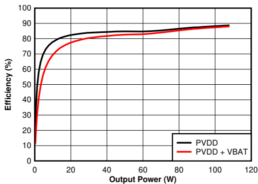
4 \Omega T_C = 75^\circ\text{C} BTL Figure 6-5. Efficiency vs Output Power - 4 \Omega
