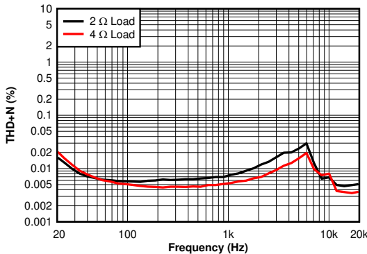
P_O = 1\text{ W} BTL Figure 6-3. THD+N vs Frequency - 2 \Omega , 4 \Omega
