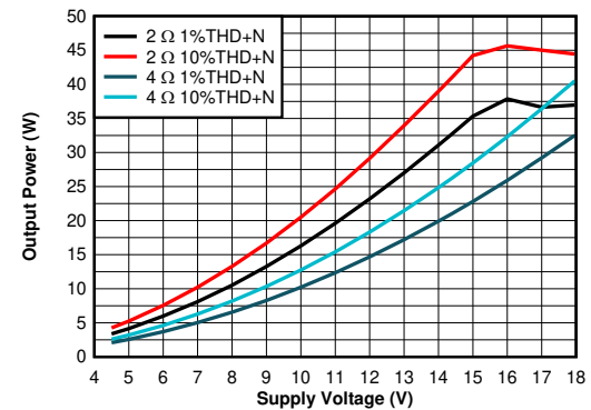
T_C = 75^\circ\text{C} BTL Figure 6-52. Output Power vs Supply Voltage - 2 \Omega 1%, 2 \Omega 10%, 4 \Omega 1%, 4 \Omega 10%
