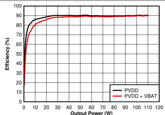
4 \Omega T_C = 75^\circ\text{C} BTL Figure 6-41. Efficiency vs Output Power - 4 \Omega
