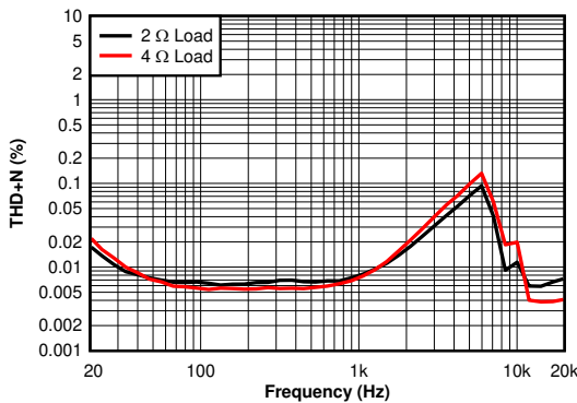
P_O = 1\text{ W} BTL Figure 6-51. THD+N vs Frequency - 2 \Omega , 4 \Omega
