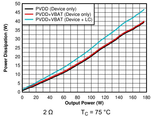
Figure 6-46. Power Dissipation vs Output Power - 2 \Omega
