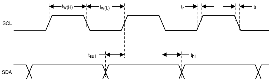
Figure 7-9. SCL and SDA Timing
