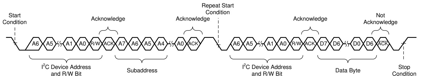
Figure 7-12. Random Read Transfer
