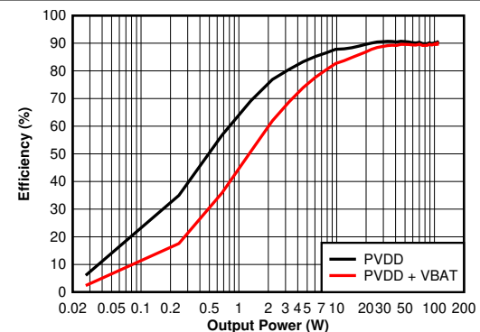
4 \Omega T_C = 75^\circ\text{C} BTL Figure 6-54. Efficiency vs Output Power - 4 \Omega (Zoomed)
