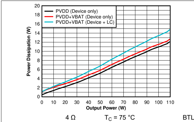
Figure 6-55. Power Dissipation vs Output Power - 4 \Omega
