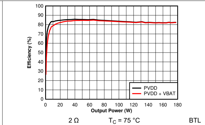
Figure 6-56. Efficiency vs Output Power - 2 \Omega
