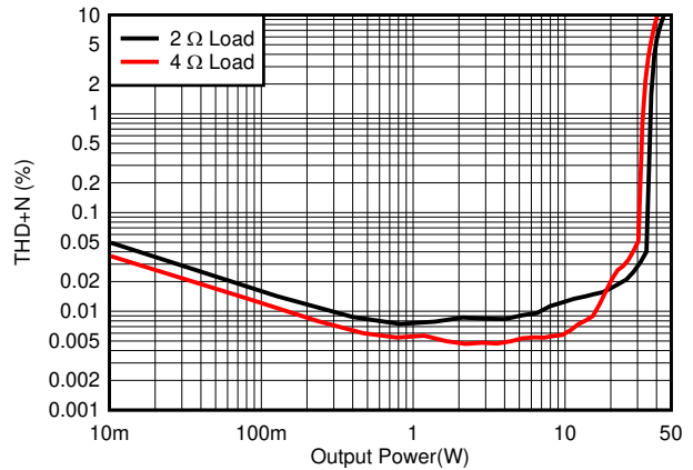
PVDD = 18V BTL Figure 6-2. THD+N vs Power - 2 \Omega , 4 \Omega - 18 V
