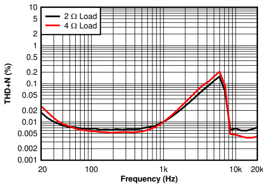
P_O = 1\text{ W} BTL Figure 6-39. THD+N vs Frequency - 2 \Omega , 4 \Omega
