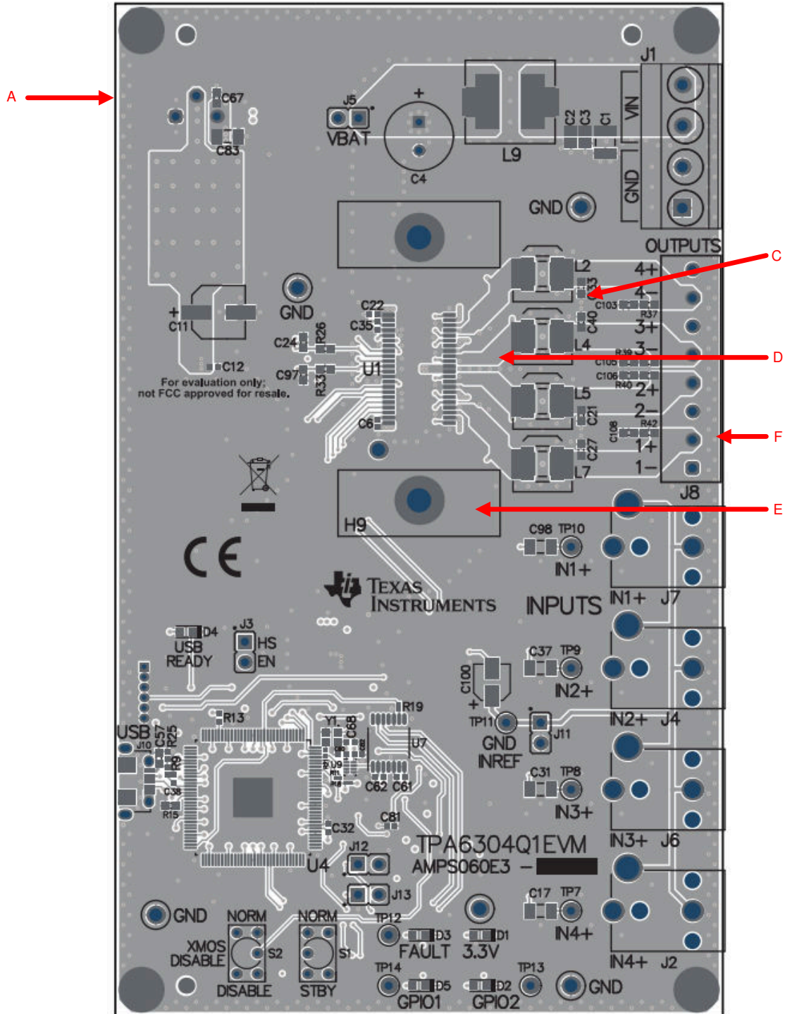
Figure 10-1. Layout Top Example
