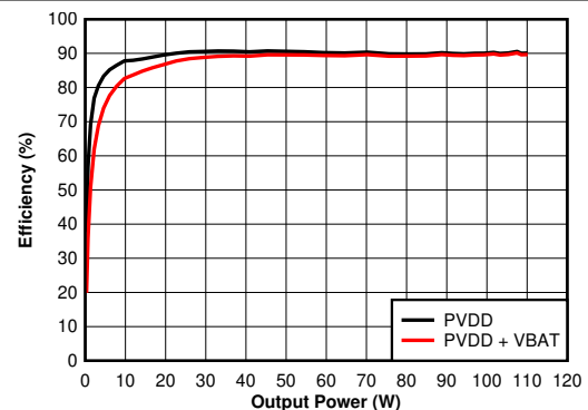
4 \Omega T_C = 75^\circ\text{C} BTL Figure 6-53. Efficiency vs Output Power - 4 \Omega
