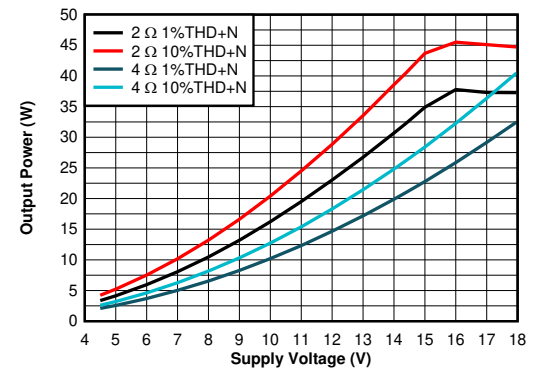
T_C = 75^\circ\text{C} BTL Figure 6-40. Output Power vs Supply Voltage - 2 \Omega 1%, 2 \Omega 10%, 4 \Omega 1%, 4 \Omega 10%
