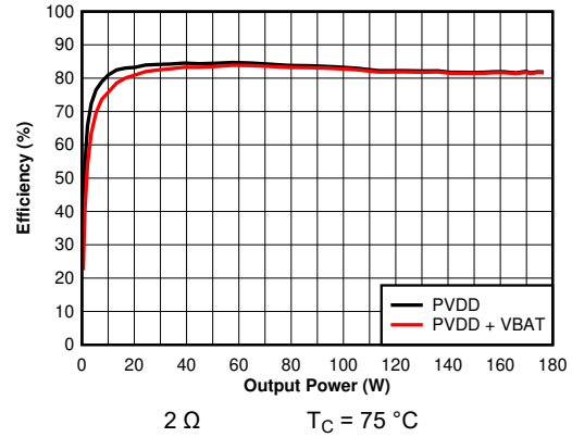
Figure 6-44. Efficiency vs Output Power - 2 \Omega
