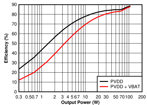
4 \Omega T_C = 75^\circ\text{C} BTL Figure 6-6. Efficiency vs Output Power - 4 \Omega (Zoomed)
