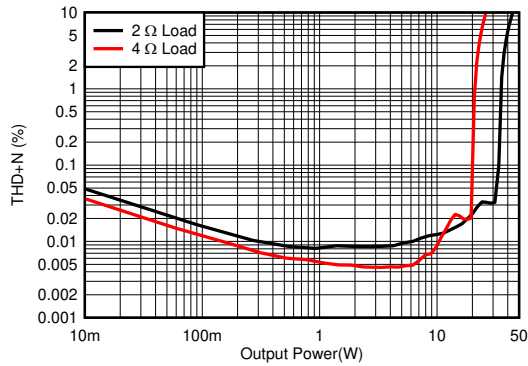
PVDD = 14.4V BTL Figure 6-1. THD+N vs Power - 2 \Omega , 4 \Omega - 14.4 V
