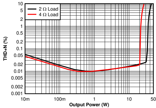
PVDD = 14.4V BTL Figure 6-37. THD+N vs Power - 2 \Omega , 4 \Omega - 14.4 V
