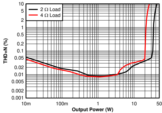
PVDD = 14.4V BTL Figure 6-49. THD+N vs Power - 2 \Omega , 4 \Omega - 14.4 V
