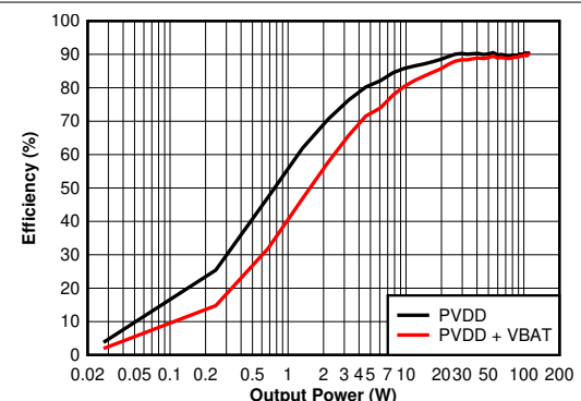
4 \Omega T_C = 75^\circ\text{C} BTL Figure 6-42. Efficiency vs Output Power - 4 \Omega (Zoomed)
