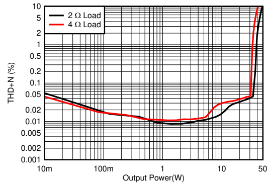
PVDD = 18V BTL Figure 6-50. THD+N vs Power - 2 \Omega , 4 \Omega - 18 V
