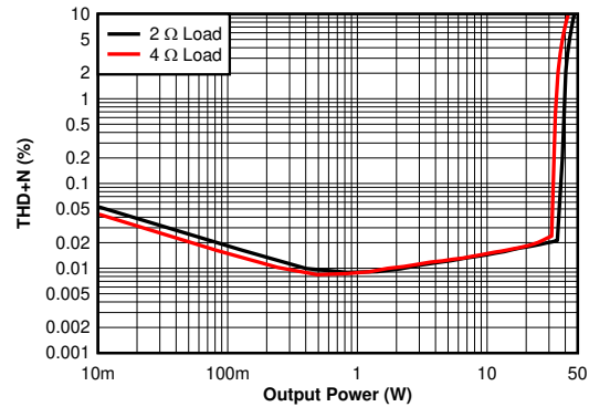
PVDD = 18V BTL Figure 6-38. THD+N vs Power - 2 \Omega , 4 \Omega - 18 V
