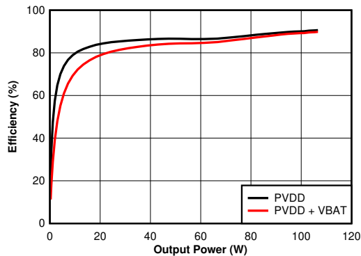
2 \Omega T_C = 75^\circ\text{C} PBTL
