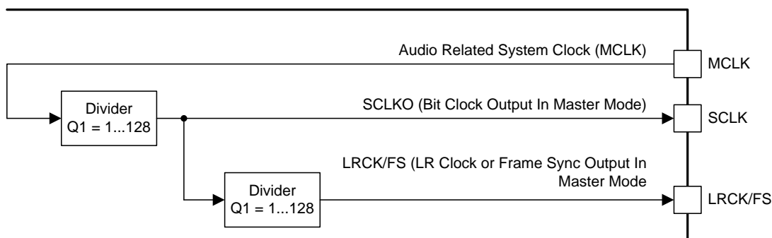
Figure 64. Simplified Clock Tree for MLCK Sourced Master Mode
