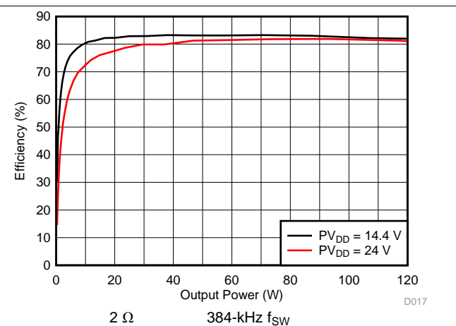
Figure 18. Power Efficiency vs Output Power
