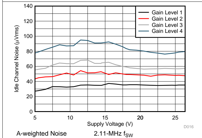
Figure 15. Noise vs Supply Voltage
