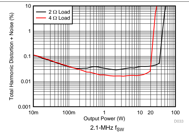
Figure 28. PBTL THD+N vs Power
