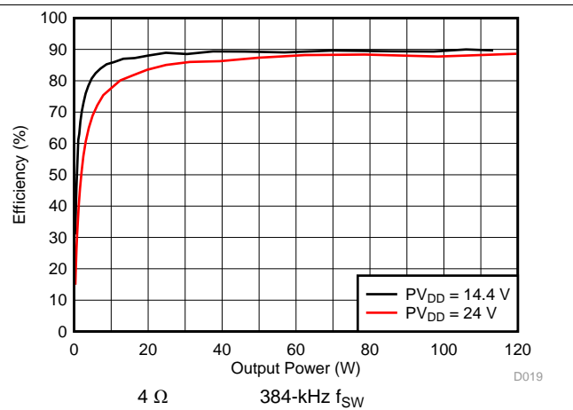
Figure 16. Power Efficiency vs Output Power
