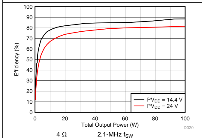
Figure 17. Power Efficiency vs Output Power
