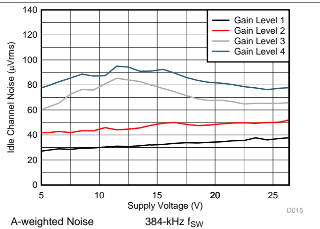
Figure 14. Noise vs Supply Voltage
