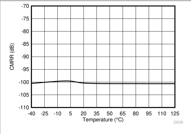
Figure 6-12. Common-Mode Rejection Ratio vs Temperature
