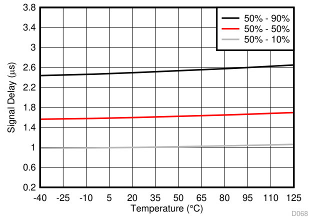
Figure 6-42. V_{IN} to V_{OUT} Signal Delay vs Temperature
