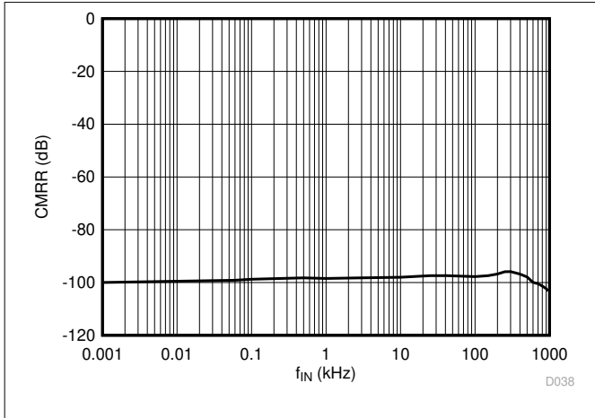
Figure 6-11. Common-Mode Rejection Ratio vs Input Frequency
