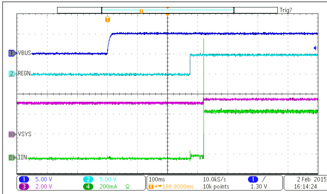
VBAT = 3.2 V I_{LIM} = 500 \text{ mA} Figure 9-2. Power Up from USB100
