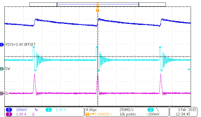
Figure 9-9. Load Transient During Supplement Mode
