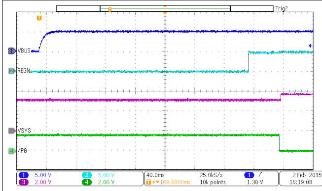
VBAT = 3.2 V Figure 9-4. Power Up with Charge Disabled
