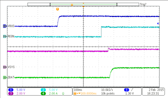
Figure 9-5. Power Up with Charge Enabled
