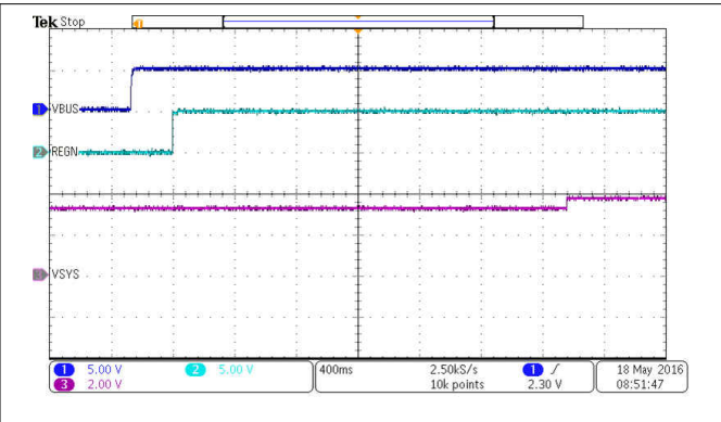
VBAT = 3.2 V Figure 9-3. Power Up with Charge Disabled
