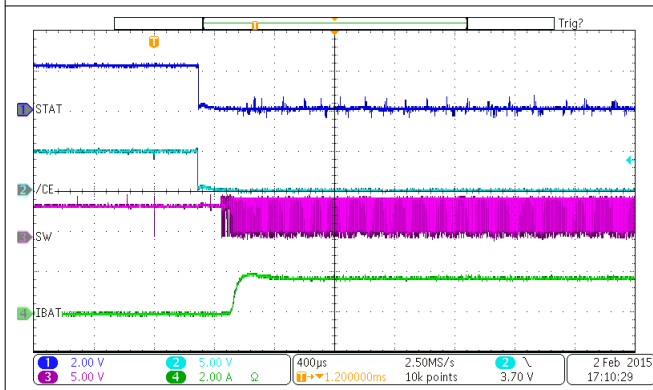
VBUS = 5 V Figure 9-6. Charge Enable
