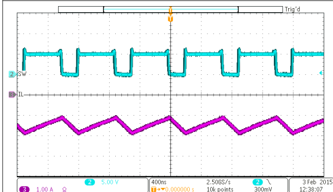
Figure 9-12. Boost Mode Switching Waveform
