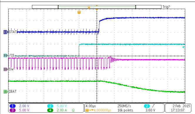
VBUS = 12 V Figure 9-7. Charge Disable
