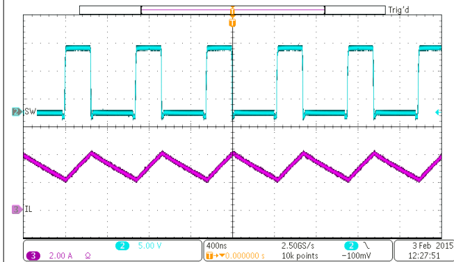
Figure 9-10. PWM Switching Waveform
