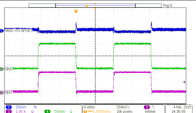
Figure 9-11. PFM Switching Waveform
