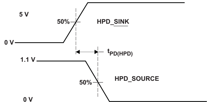
Figure 9. HPD Timing Diagram (HPDINV = HIGH)
