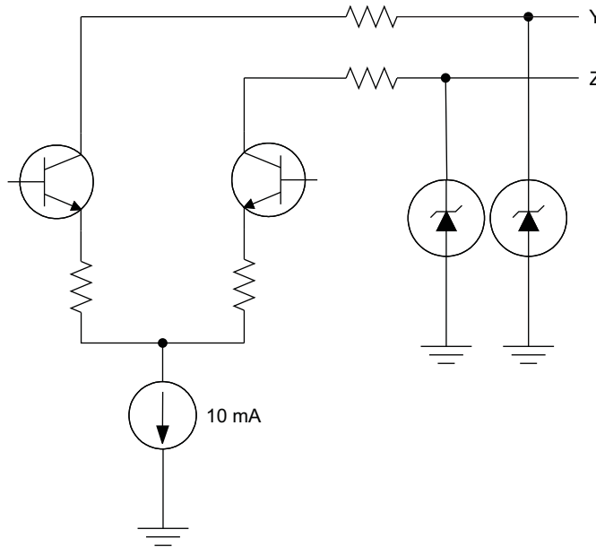
Figure 2. TMD5 Output Stage
