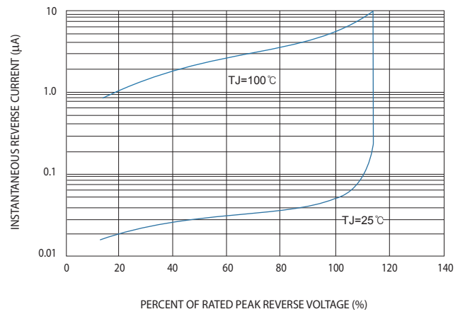
FIG.4-TYPICAL REVERSE CHARACTERISTICS
