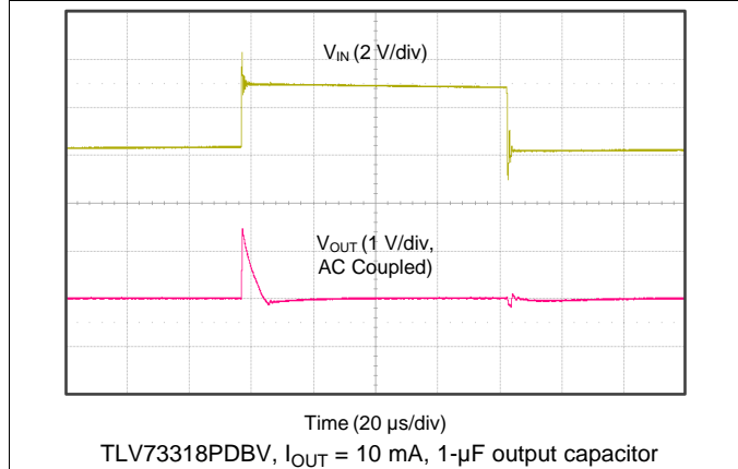
Figure 23. Line Transient
