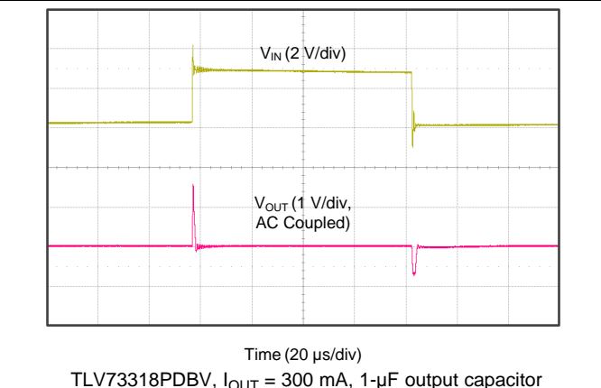
Figure 24. Line Transient
