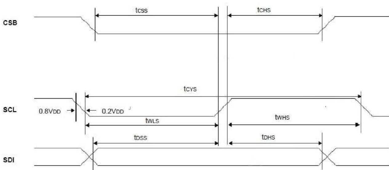
Serial Bus Timing Characteristics (for Serial MCU)
