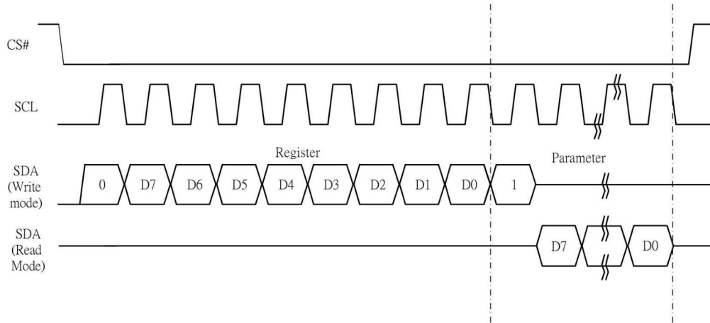
Figure 6-4: Read procedure in 3-wire SPI mode
