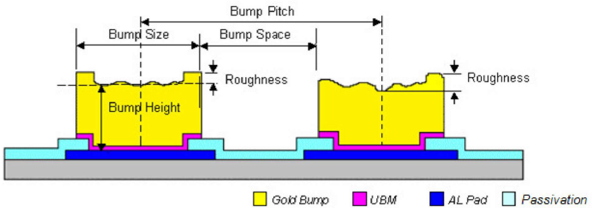
Bump Height Coplanarity within Die
