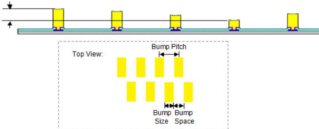
Bump Height Coplanarity within Die
