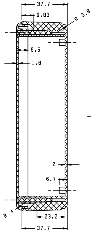
SECTION J - J
