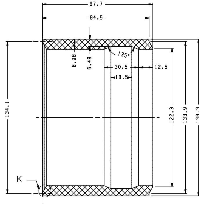
SECTION J - J
